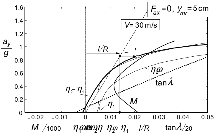
Fig. 11.28. The handling diagram at zero forward acceleration with 5cm lateral shift of the centre of gravity of combined rider and mainframe mass ( V = 108 km/h).
