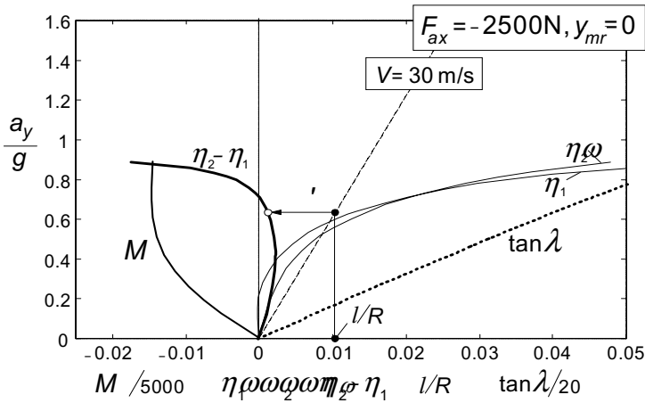
Fig. 11.27. The handling diagram at hard braking ( V = 108 km/h).
