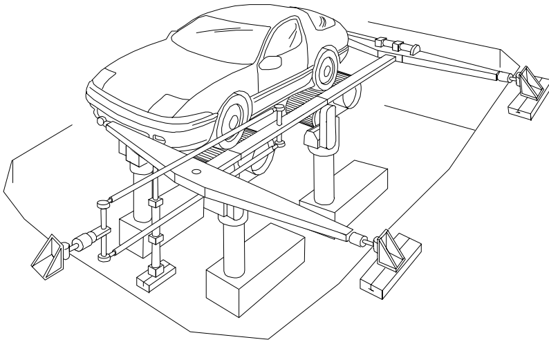
Fig. 1.28. The MTS Flat-Trac Roadway Simulator TM , Milliken (1995).
