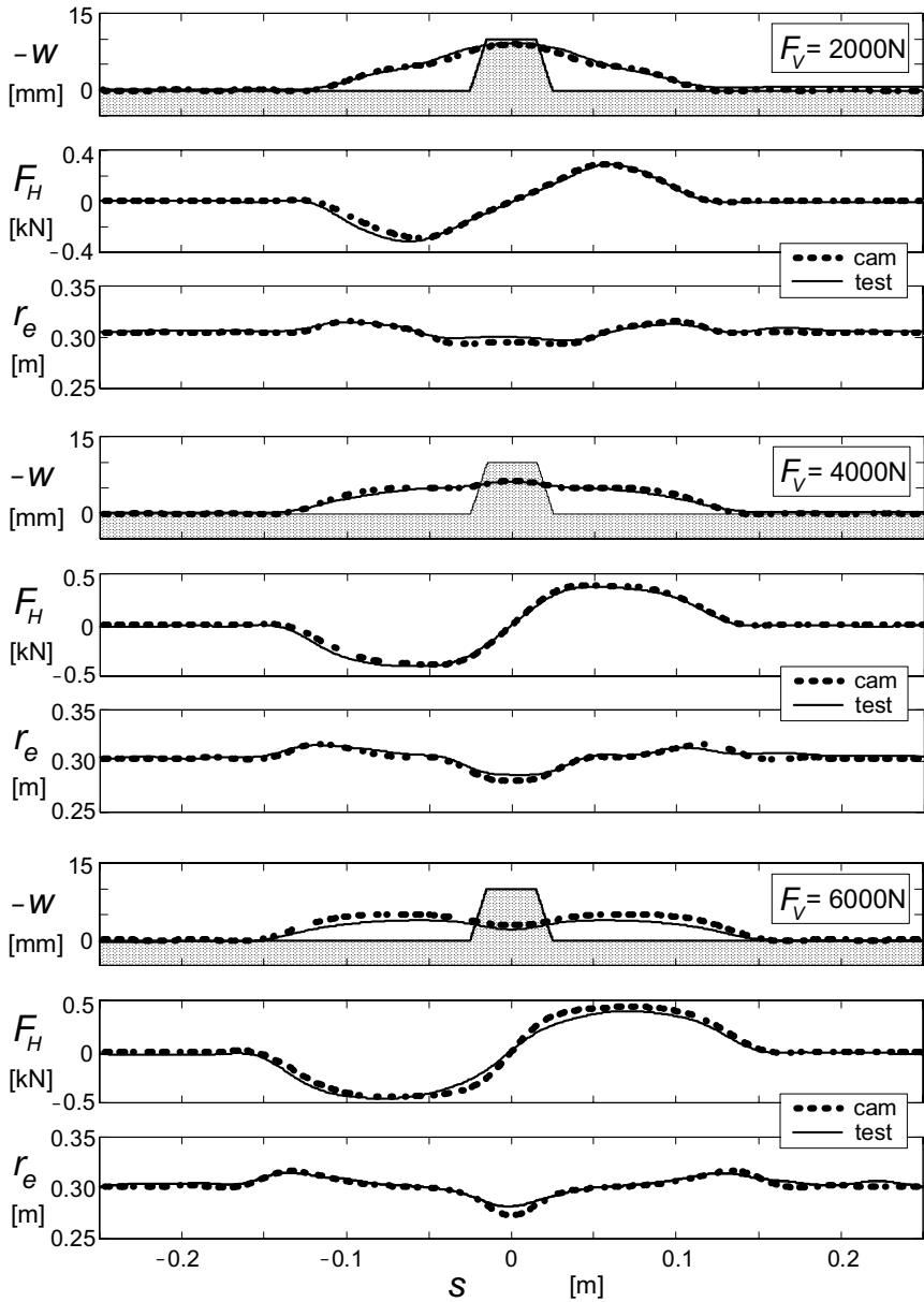
Fig. 10.18. Rolling over a trapezium cleat (length: 50mm, height: 10mm). Measured and calculated variation of vertical axle displacement, horizontal longitudinal force and effective rolling radius at three different constant vertical loads. Measurements carried out on the Delft flat plank machine (very low speed) and calculations conducted with the use of the tandem cam technique (Fig. 10.11) and Eq. (10.22). Tandem cam parameters according to Table 10.1.
