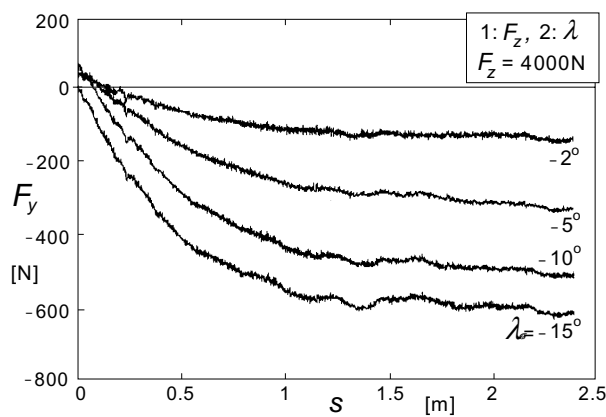
Fig. 7.11a. Side force response to step change in camber angle.
