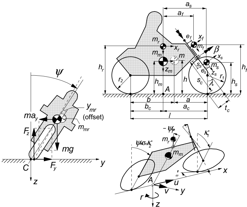
Fig. 11.1. Motorcycle model configuration.
