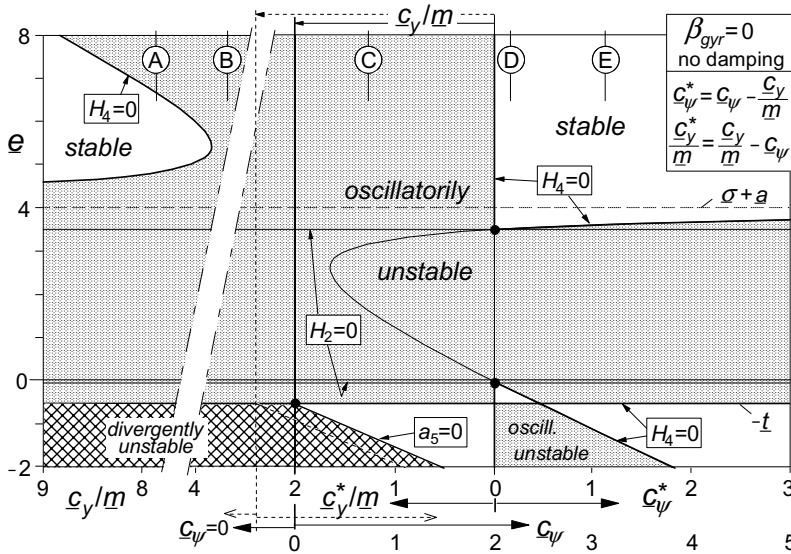
Fig. 6.10. Basic stability diagram according to conditions (6.46-48) for the fifth-order system without damping and gyroscopic coupling. The diagram hold in general, the case with \underline{c}_y/\underline{m} = 2 is an example, note: \underline{m} = 0.5 .
