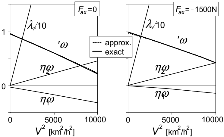
Fig. 11.17. Steer, roll and slip angles per unit non-dimensional path curvature l/R vs speed squared V^2 = a_x R (left: non-accelerating, right: braking) according to the exact and approximate theories.
