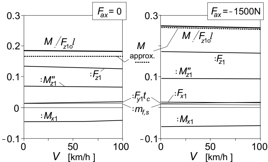
Fig. 11.21. The non-dimensional steer torque ( M_\delta/(F_{z10}I) ) and its components (cf. Eq.(11.147)) per m.c.g. lateral offset y_{mv} . In M''_z the F_{x1} contribution is removed.
