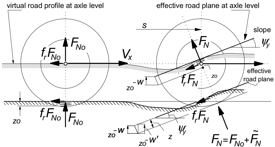
Fig. 10.5. The virtual road profile and effective road plane as sensed at wheel axle level.
