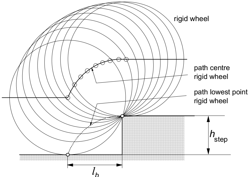
Fig. 10.8. The rigid wheel rolling over an upward step change in road level.
