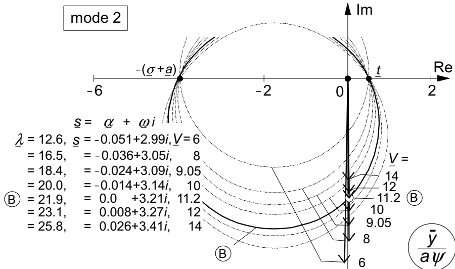
Fig. 6.23. Circles and phasors of mode shapes of mode 2 for same series of speed values as in Fig.6.22. At increasing speed the phasor crosses the circle at \underline{V} = 11.2 towards its inside which means: entering the unstable domain.
