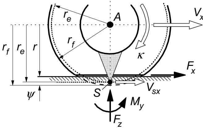
Fig. 2.4. Effective rolling radius and longitudinal slip velocity.
