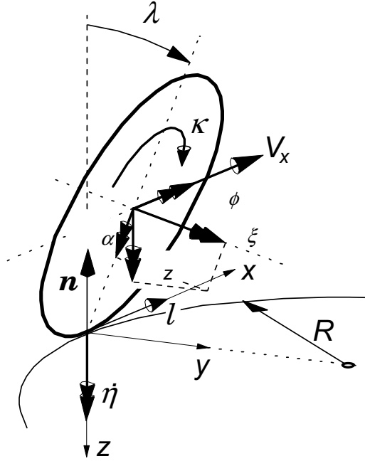
Fig. 2.6. Rotational slip resulting from path curvature and wheel camber (slip angle = 0).
